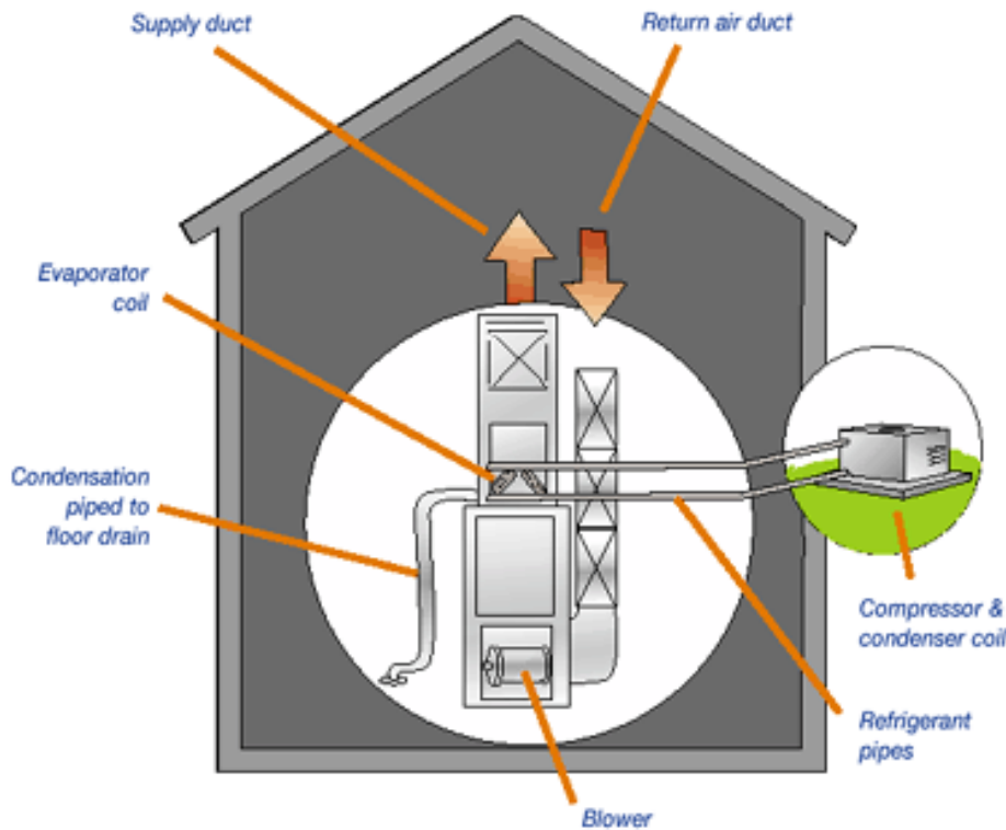
Central Air Conditioner on a Forced Air System
